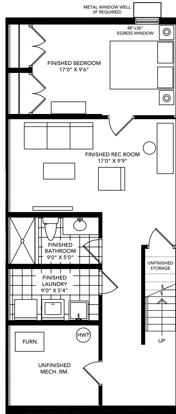
OPTIONAL FINISHED BASEMENT 645 SQ. FT.
